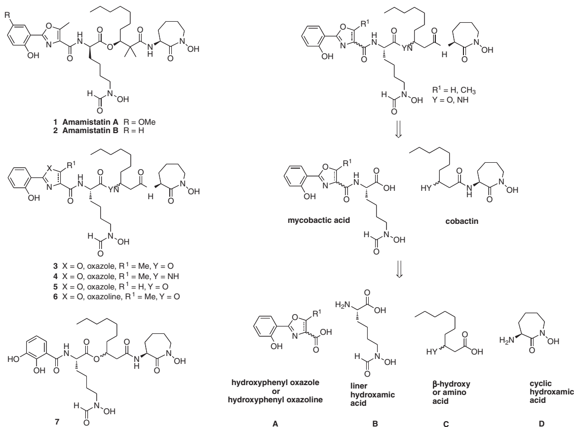
Figure 1. Amamistatins, analogs and their retro-synthetic analysis.
